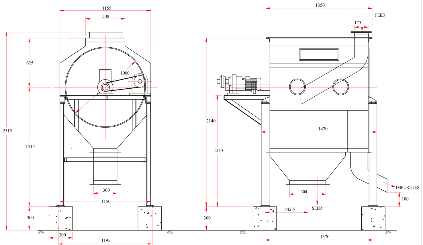
DRUM SIEVE CORSE CLEANER
