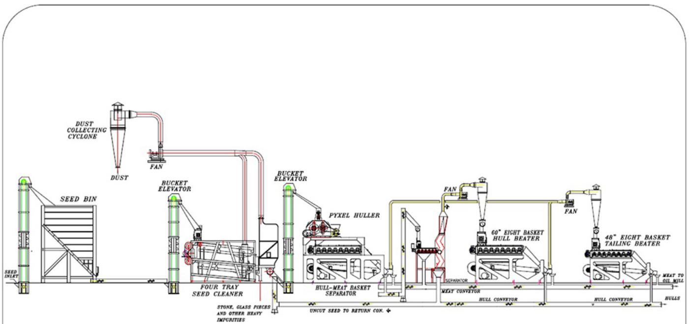
FLOW DIAGRAM FOR SUNFLOWER SEED CLEANING & HULLING PLANT
